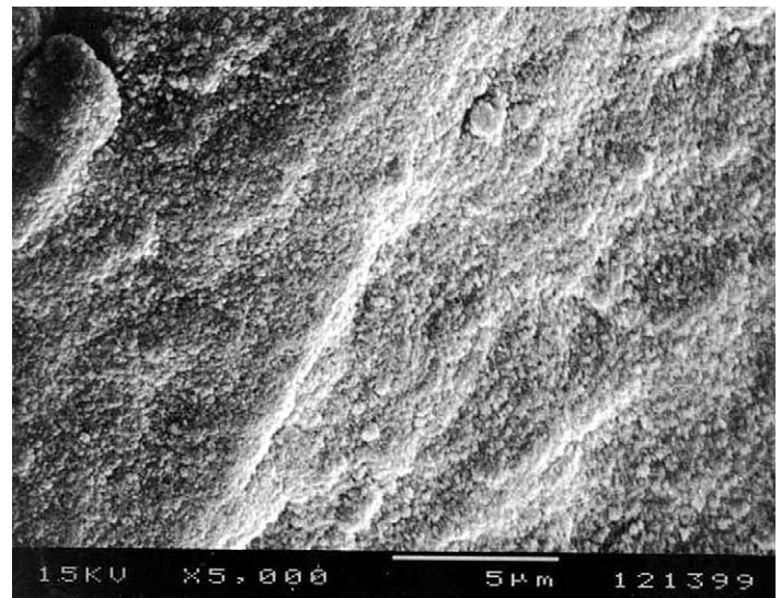
Material: 50 µm 75% Nickel / Graphite 25% (single particle) Surface Area: 0.19 m 2 /g Original Magnification: 5000X
