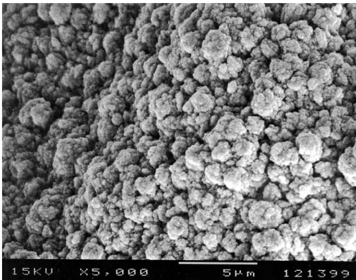
Material: 50 µm 75% Nickel / Graphite 25% (single particle) Surface Area: 1.28 m 2 /g Original Magnification: 5000X
